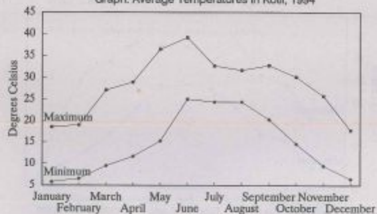
Graph. Average Temperatures in Kotli, 1994
